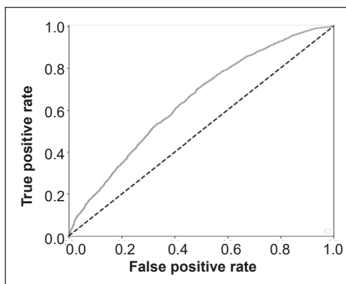
Figure 5. ROC characteristics of Higgs dataset
