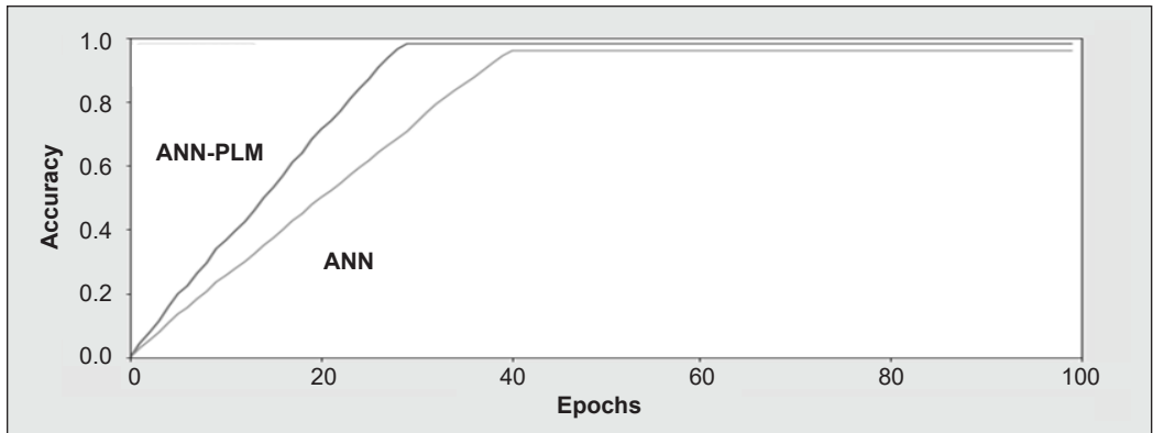
Figure 8. Convergence graph of Higgs dataset with ANN and ANN-PLM
